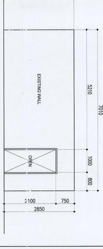
PLAN: PARTITION F SCALE: 1:60
