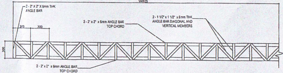
ROOF BEAM DETAIL N T S
