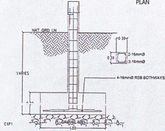
COLUMN & FOOTING DETAIL N T S
