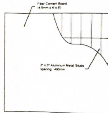
TYPICAL PARTITION DETAILS N.T.S.
