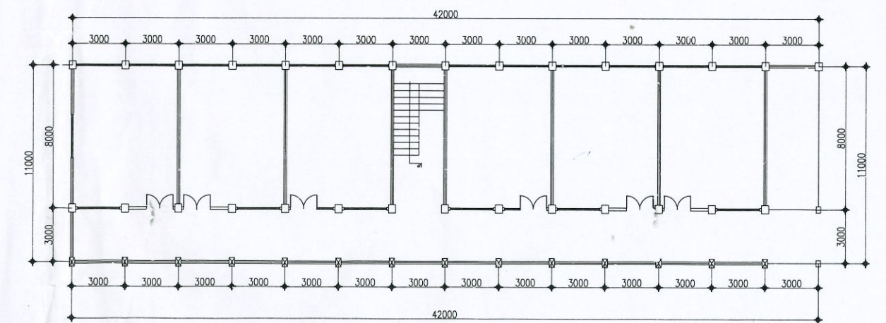
SECOND FLOOR PLAN SCALE: 1:100
