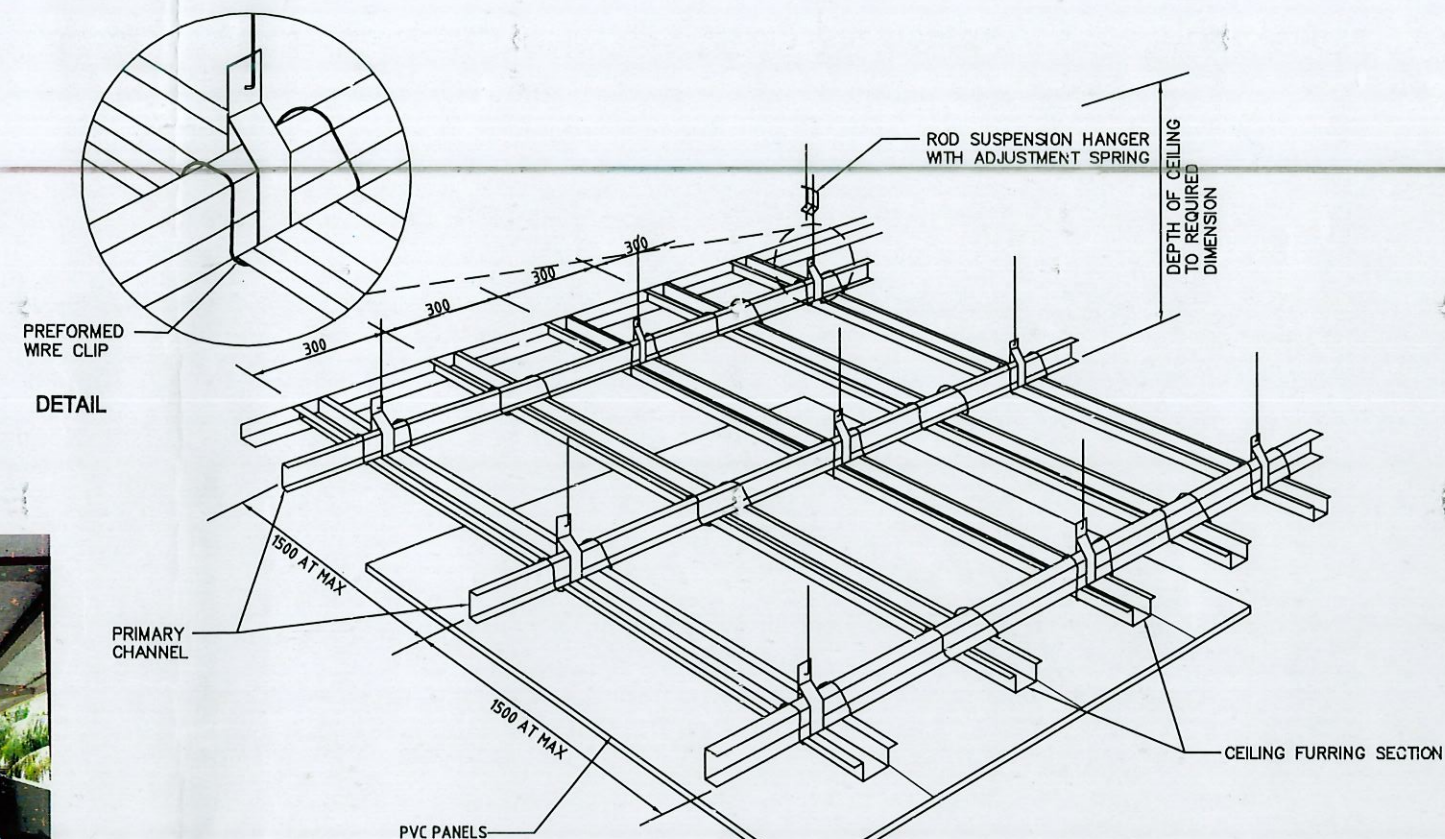
4 CEILING PERSPECTIVE/DETAIL A-1 NTS
