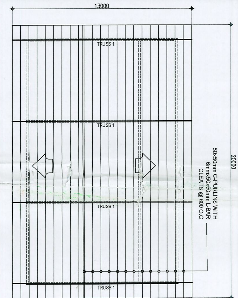
ROOF FRAMING PLAN NTS
