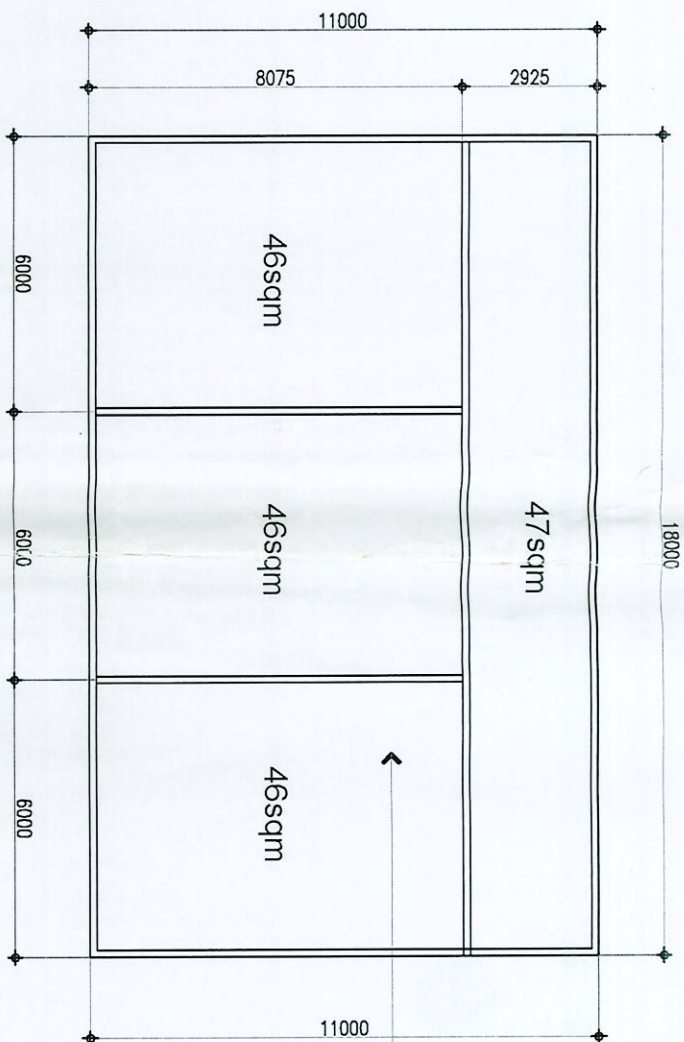
CEILING PLAN NTS
